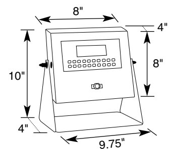
5900 Series Indicator
